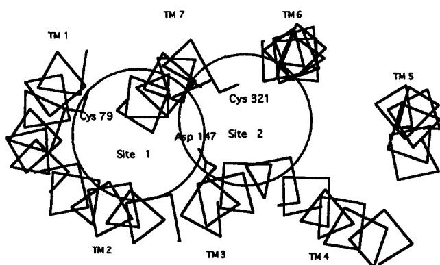
Figure 8. View of the \mu -opioid receptor model (extracellular view). Putative binding sites 1 and 2 are indicated.
