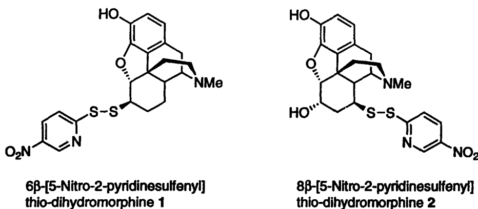
Figure 4. Structure of 6 \beta -[5-nitro-2-pyridinesulfonyl] thio-dihydromorphine and 8 \beta -[5-nitro-2-pyridinesulfonyl] thio-dihydromorphine.
