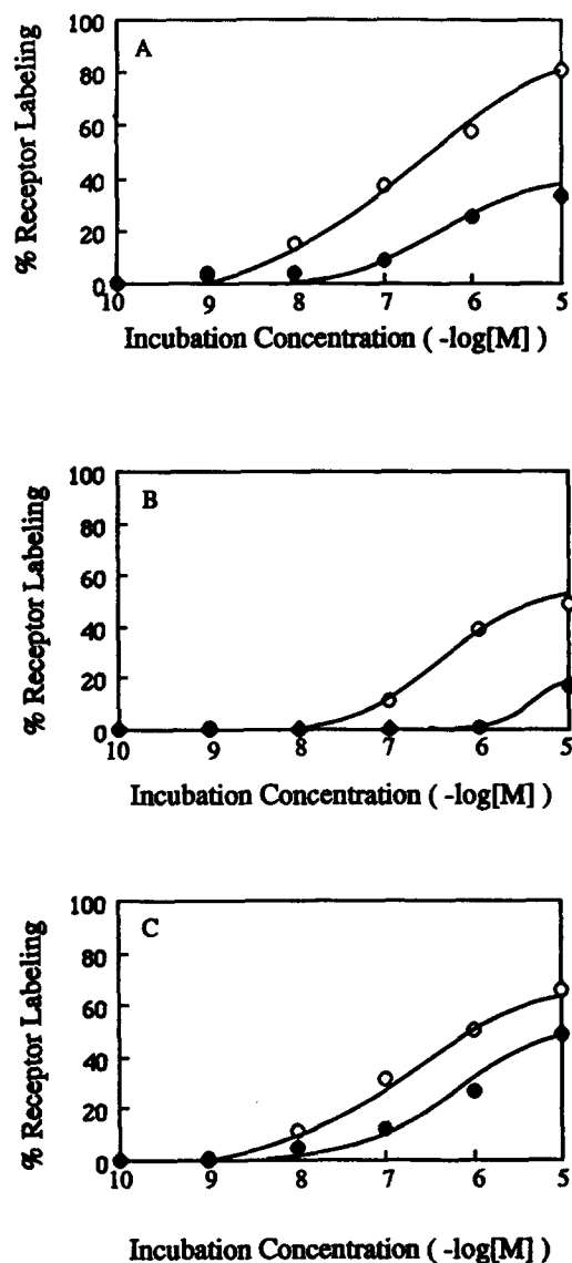
Figure 7. The concentration-dependent affinity labeling of \mu (A), \delta (B) and \kappa (C) opioid receptors by S -activated ligands. Compounds 1 (○—○) and 2 (●—●).
