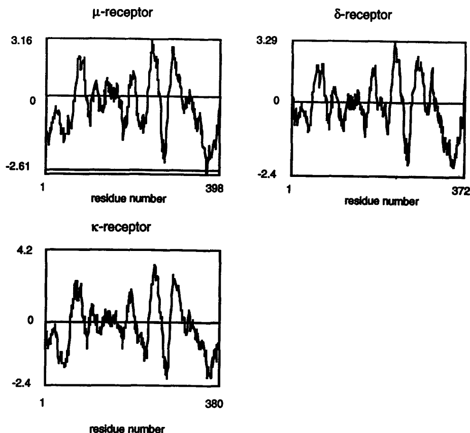
Figure 2. Hydrophilicity/hydrophobicity plots of opioid receptors. Parameter: Kyte & Doolittle. Range to average: 15.
